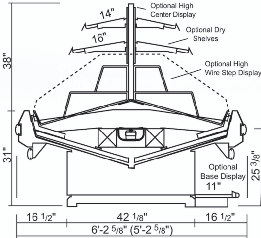
DSRPI-03 Shelf & Rack Option
