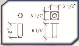
BULLET FEET / OPTIONAL LEGS
