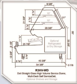
R3HV-WD - STRAIGHT GLASS
