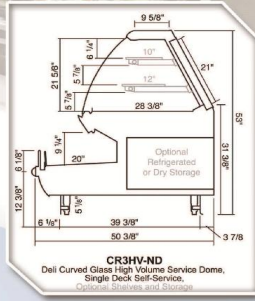
CR3HV-ND - CURVED GLASS
