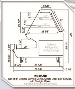
R3HV-ND - STRAIGHT GLASS
