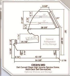
CR3HV-WD - CURVED GLASS
