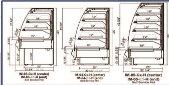
IM-H Isla Module: Multi Deck Hot Display!
