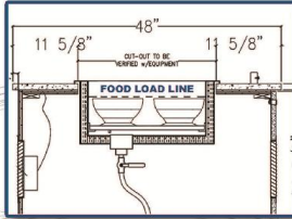
PRODUCT VISIBILITY 3" BELOW COUNTER DISPLAY
