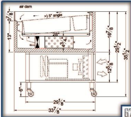
VIAP4-0-R-SC (SLANT EXTRA DEEP)
