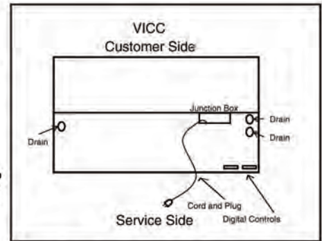
Electrical & Plumbing locations
