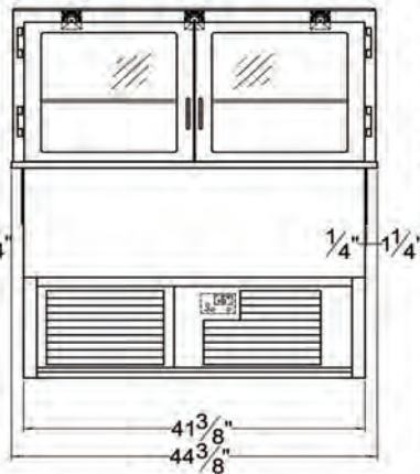
VICD3(A)-R-CV-SC FD
