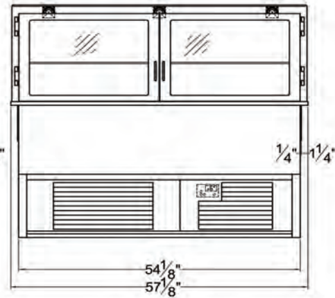
VICD4(A)-R-CV-SC FD
