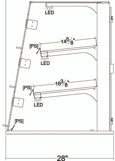
side elevation
