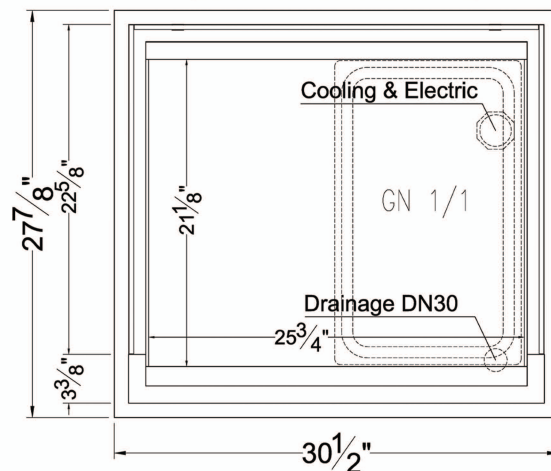
Electrical & Plumbing locations
