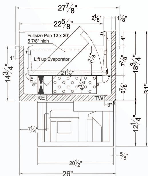
Gross Section
