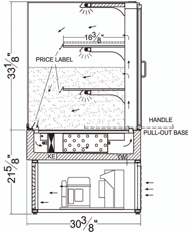
(SECTION VIEW SIDE)
