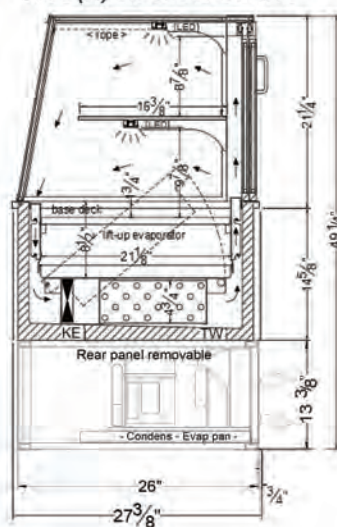
VICD(A)-20-R-SL-SC INS
