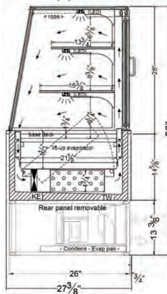
VICD(A)-27-R-SL-SC INS
