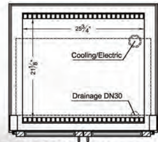
Electrical & Plumbing locations
